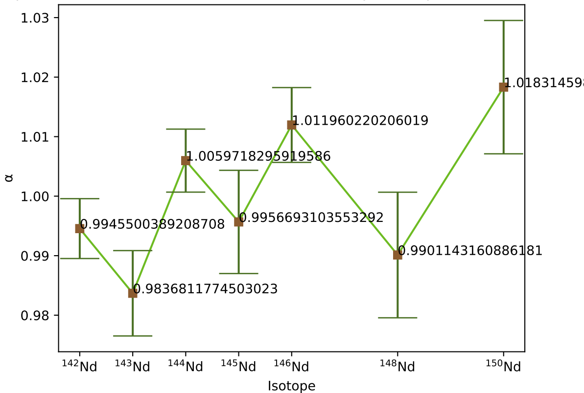
Alpha Coefficient Trends as a Function of Isotopic Composition 07/02/2024
