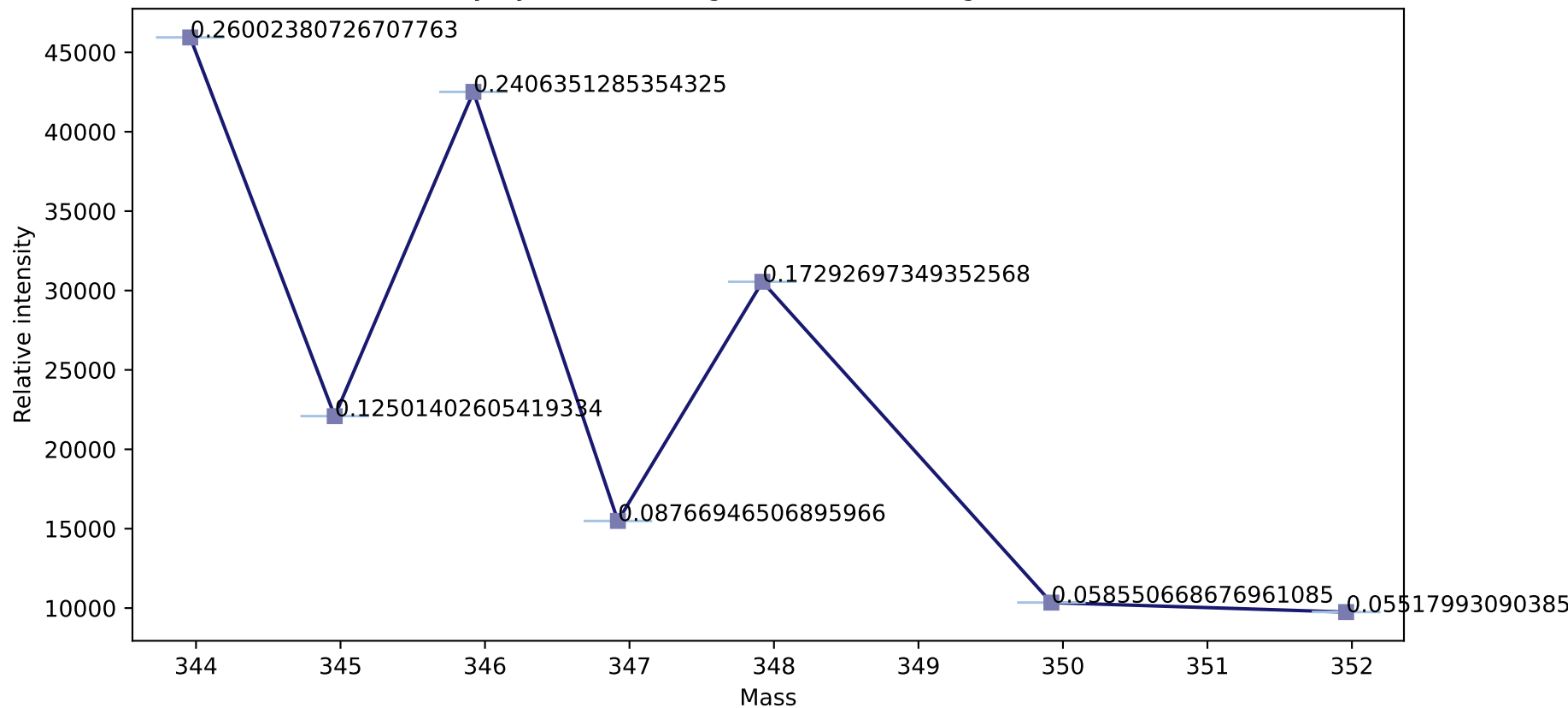
Relative Intensity by Mass in Daughter Molecule Fragmentation 07/02/2024
