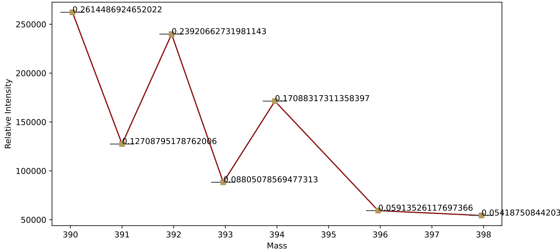
Relative Intensity by Mass in Parent Molecule Fragmentation 07/02/2024
